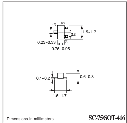
SC-75/SOT-416
