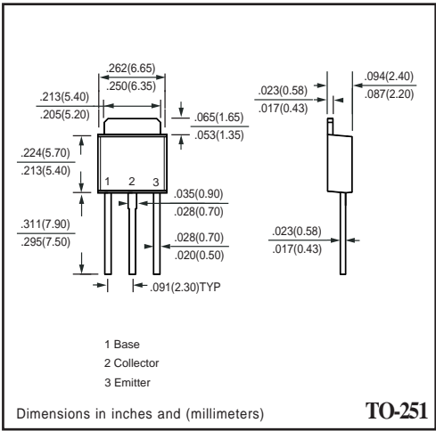
TO-251
