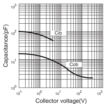
Fig.4 Capacitance
