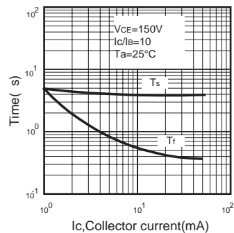
Fig.3 Turn-off switching times
