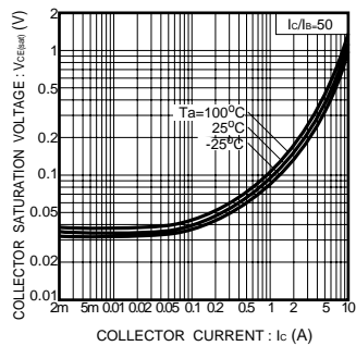
Fig.7 Collector-emitter saturation voltage vs. collector current ( V )
