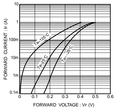
Fig.8 Forward characteristics
