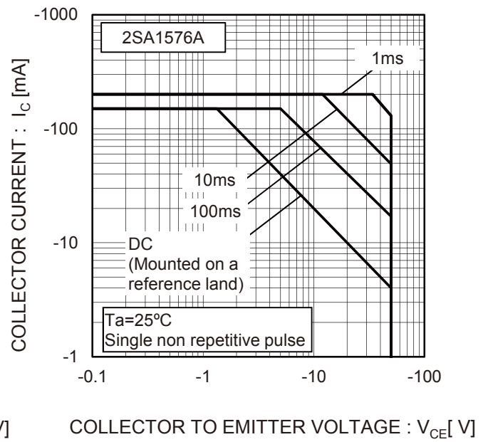
Fig.14 Safe Operating Area
