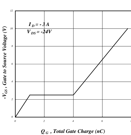
Fig 7. Gate Charge Characteristics
