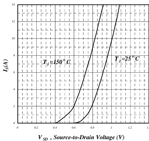
Fig 5. Forward Characteristic of the Reverse Diode
