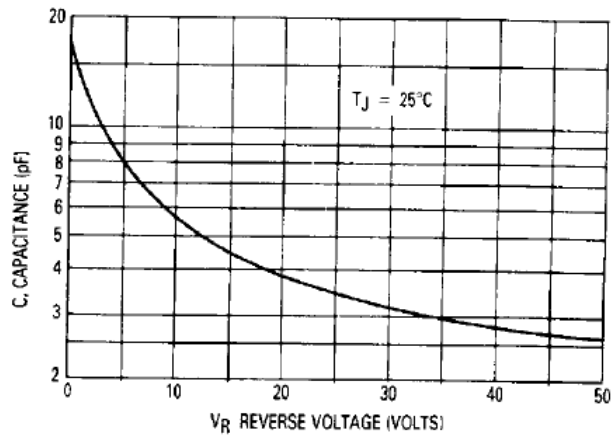
Figure 5. Typical Capacitance
