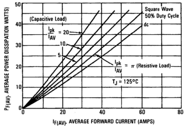
FIGURE 6 — POWER DISSIPATION
