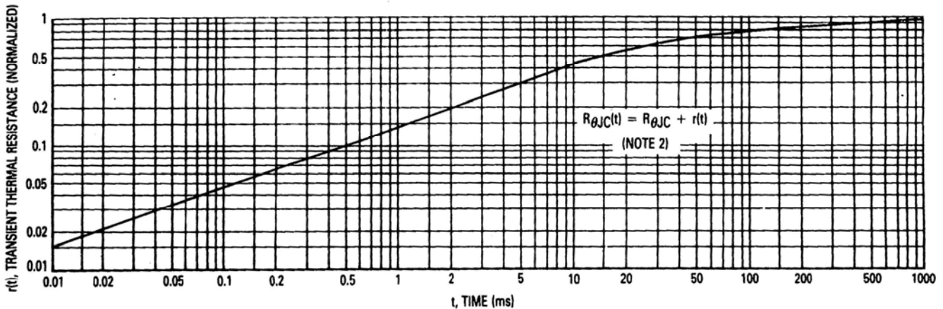
Figure 7. Thermal Response
