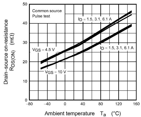
Fig. 8.2.6 R_{DS(ON)} - T_a
