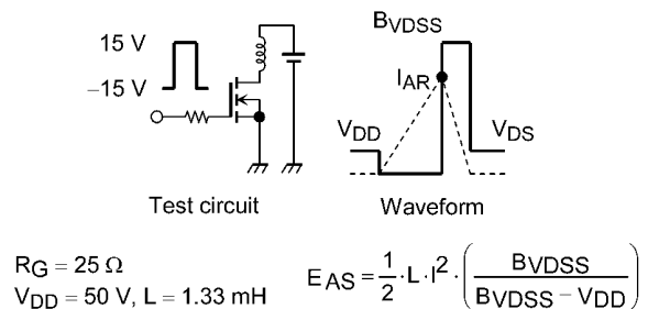
Fig. 8.16 Test Circuit/Waveform
