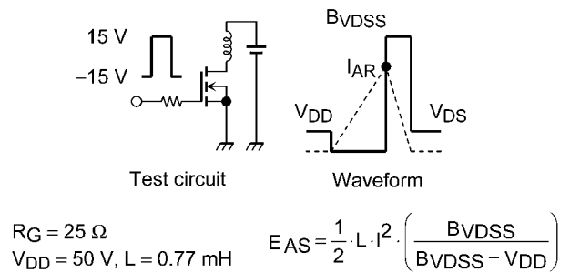
Fig. 8.16 Test Circuit/Waveform
