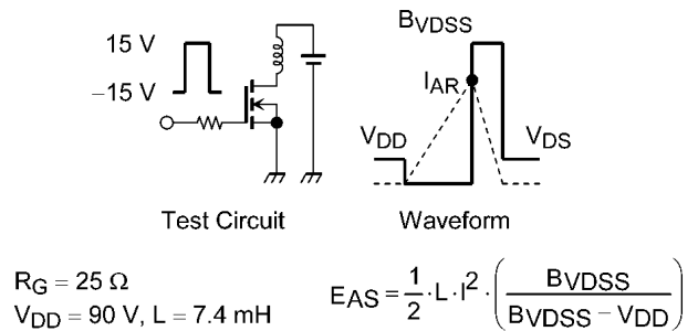
Fig. 8.16 Test Circuit/Waveform
