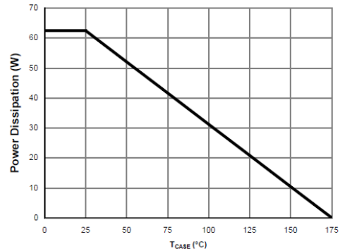
Figure 13: Power De-rating (Note B)
