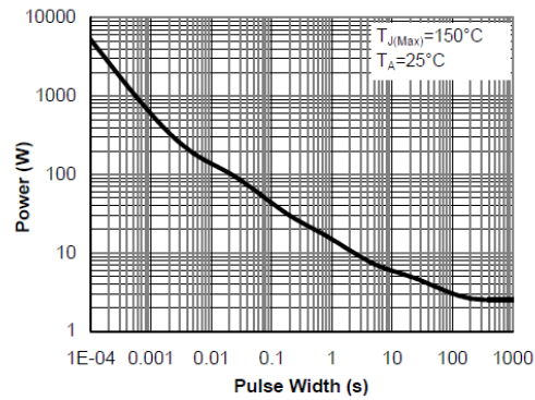
Figure 15: Single Pulse Power Rating Junction-to-Ambient (Note G)
