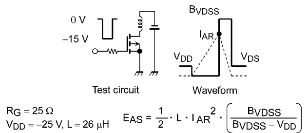
Fig. 9.15 Test Circuit/Waveform
