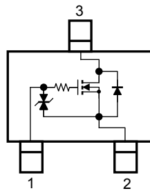
Equivalent Circuit (top view)
