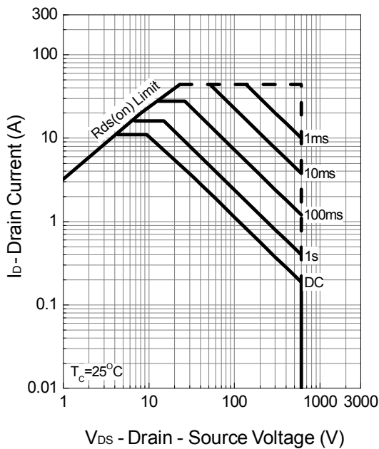
Safe Operation Area : TO-220/TO-251
