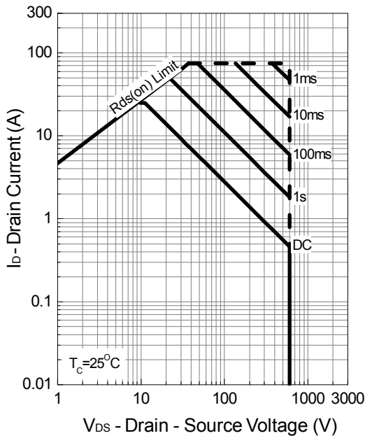
Safe Operation Area : TO-220
