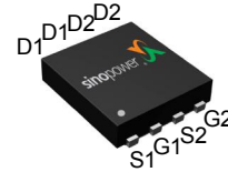
Top View of DFN3x3-8
