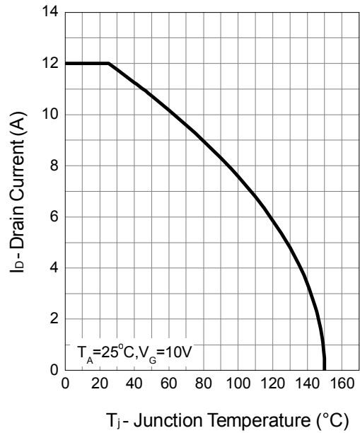
Drain Current
