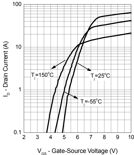
Transfer Characteristics
