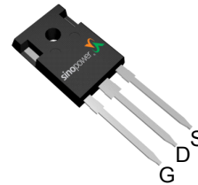
TO-247
