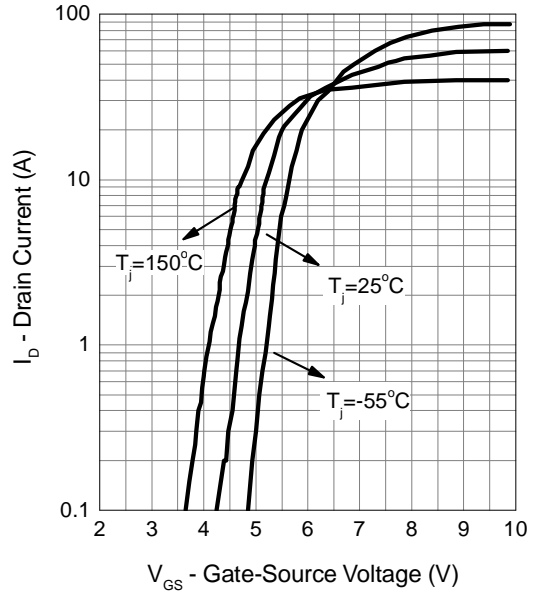
Transfer Characteristics
