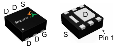
DFN2x2-6
