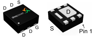
DFN2x2-6
