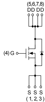
N-Channel MOSFET
