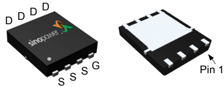
DFN5x6-8
