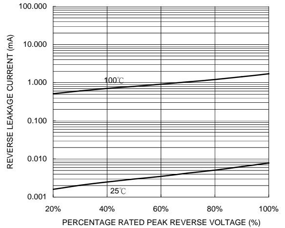
FIG. 4-TYPICAL REVERSE CHARACTERISTICS
