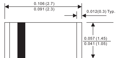
SOD-323-L
