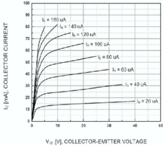
Fig.1 Static Characteristic
