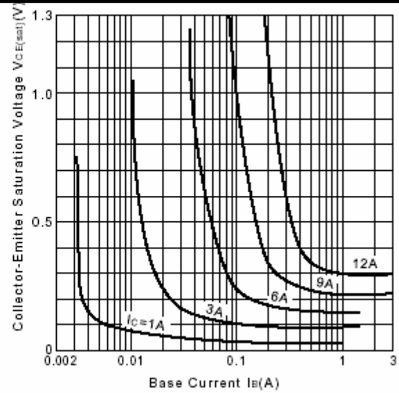
Fig.4 V_{CE(sat)}-I_B Characteristics
