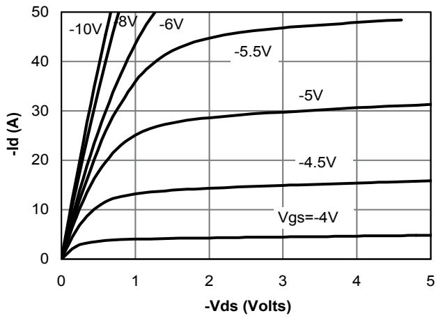
Fig 1: On-Region Characteristics
