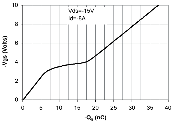
Figure 7: Gate-Charge Characteristics
