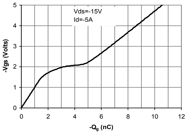
Figure 7: Gate-Charge Characteristics
