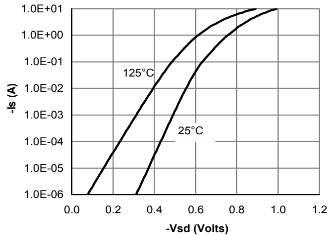
Figure 6: Body-Diode Characteristics
