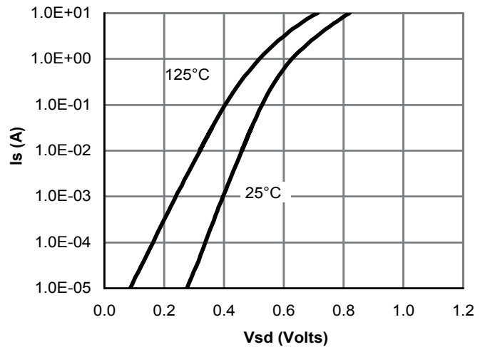
Figure 6: Body-Diode Characteristics
