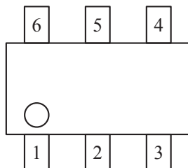
SOT-26(TOP VIEW)
