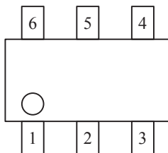
SC-70-6(TOP VIEW)
