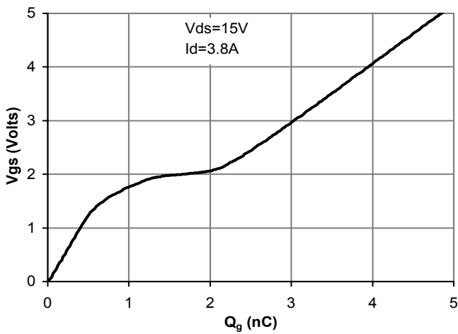
Figure 7: Gate-Charge Characteristics
