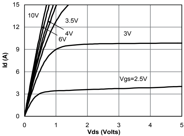
Fig 1: On-Region Characteristics
