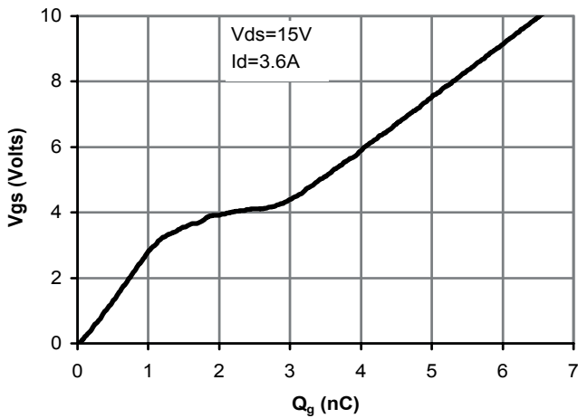
Figure 7: Gate-Charge Characteristics
