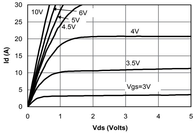
Fig 1: On-Region Characteristics
