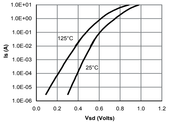
Figure 6: Body-Diode Characteristics
