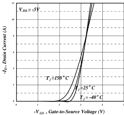
Fig 11. Transfer Characteristics
