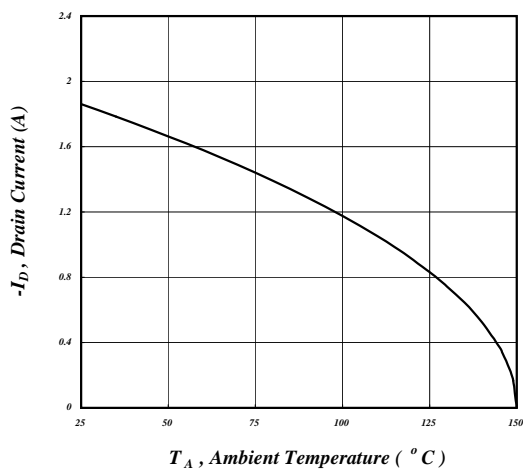
Fig 11. Drain Current v.s. Ambient Temperature (Note3)
