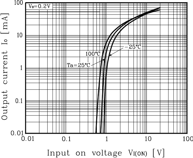
Fig. 1 I_O - V_{I(ON)}
