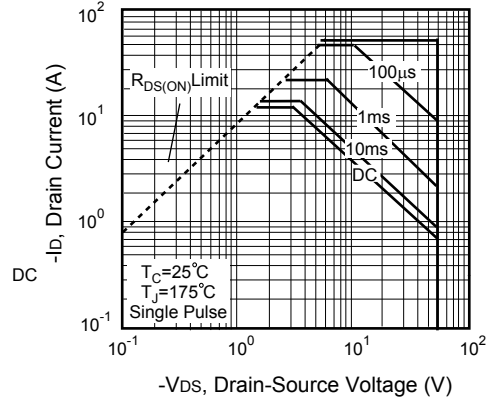
Figure 8. Maximum Safe Operating Area
