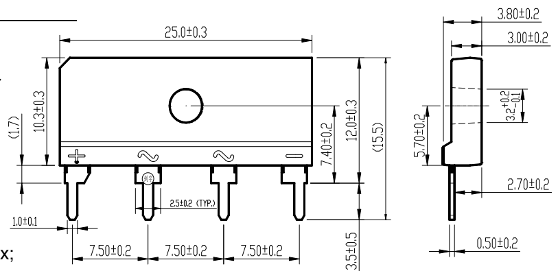
Package Dimensions in mm
