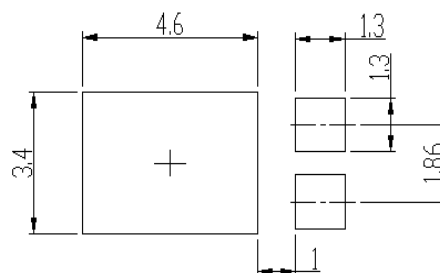
Soldering footprint
