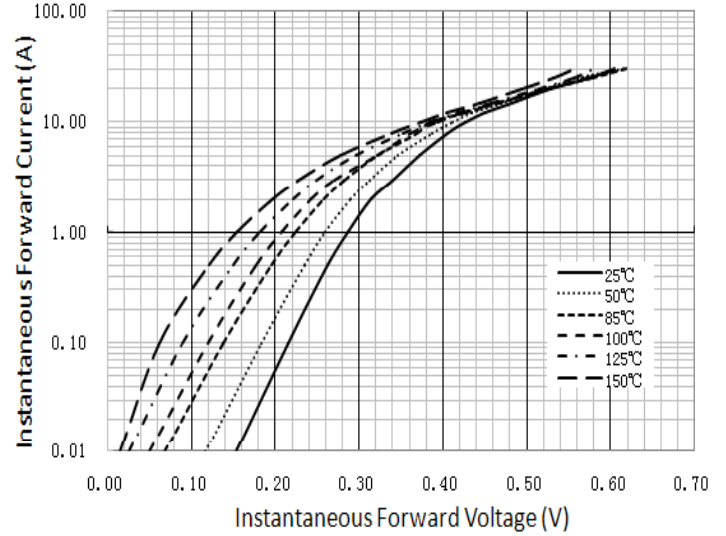
Figure 2. Typical Instantaneous Forward Characteristics
