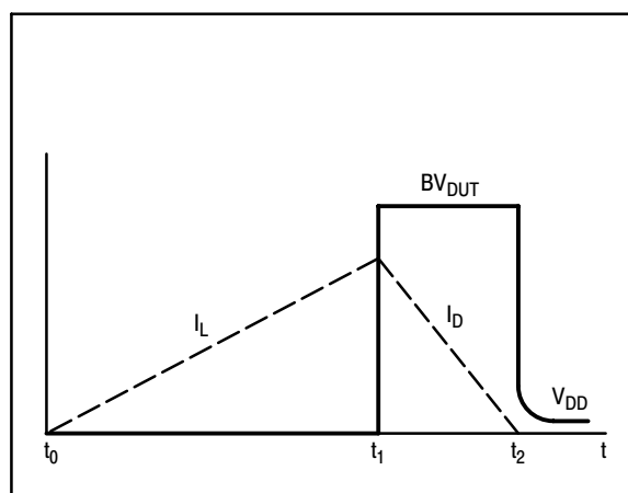
Figure 11. Current-Voltage Waveforms
